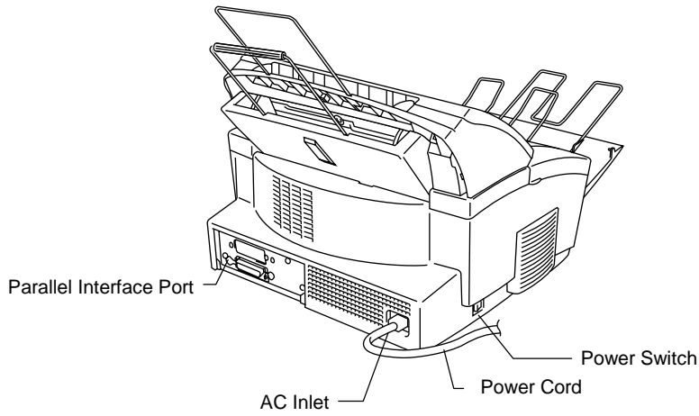
Fig. 1-2 Rear View
